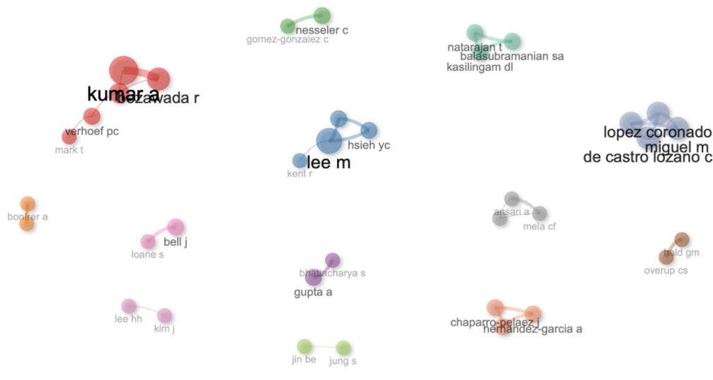
Figure 6. Collaboration Network
