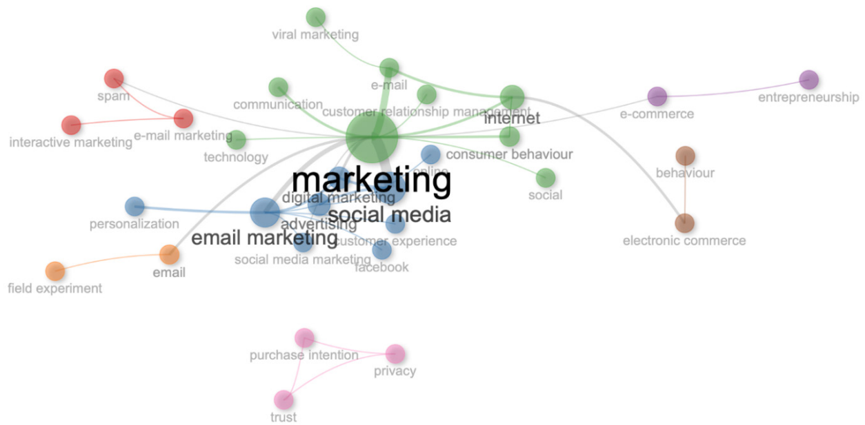
Figure 9. Co-occurrence Map
